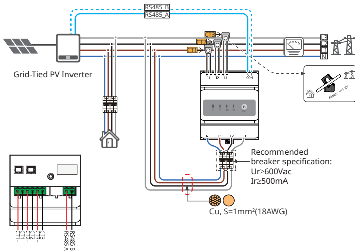
Type I: Three-phase four-wire
